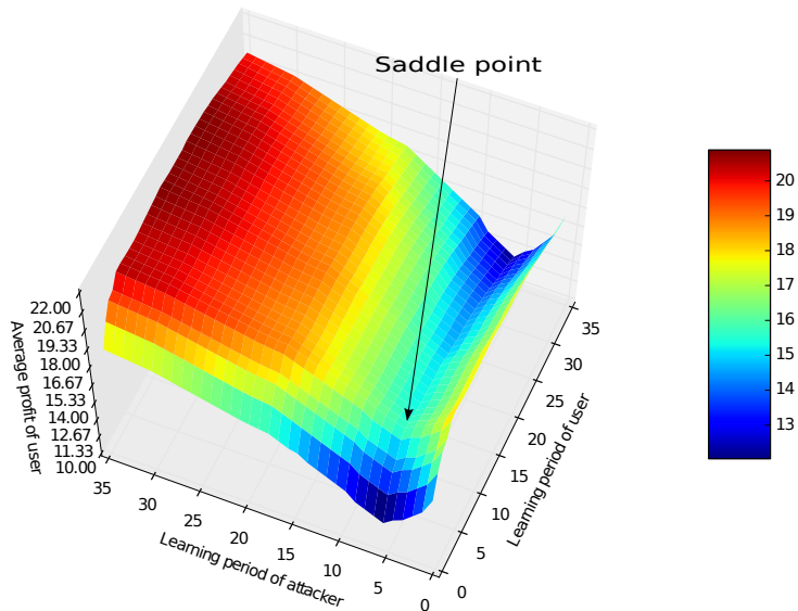
Figure 4: Saddle point for learning period
