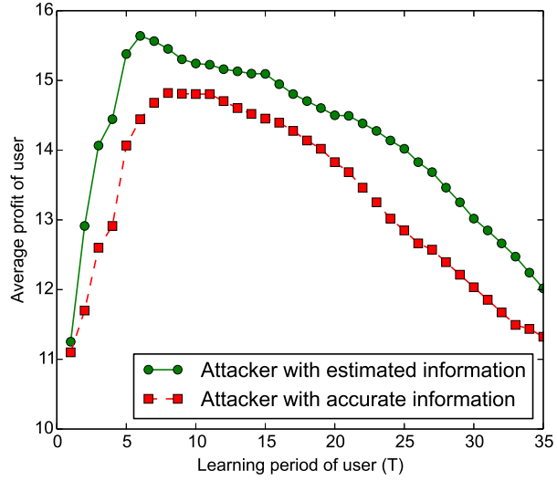
Figure 5: Performance when attacker has estimated/accurate information. The learning time for attacker is fixed.
