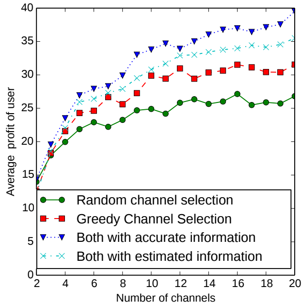
Figure 6: Comparison of average profit to Random and Greedy benchmarks
